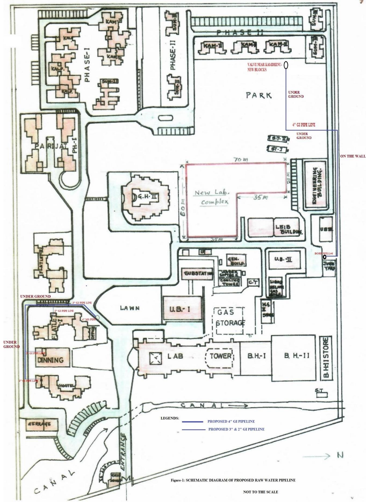
FIG.1 SCHEMATIC DIAGRAM OF INDICATIVE WATER PIPELINE LAYOUT
