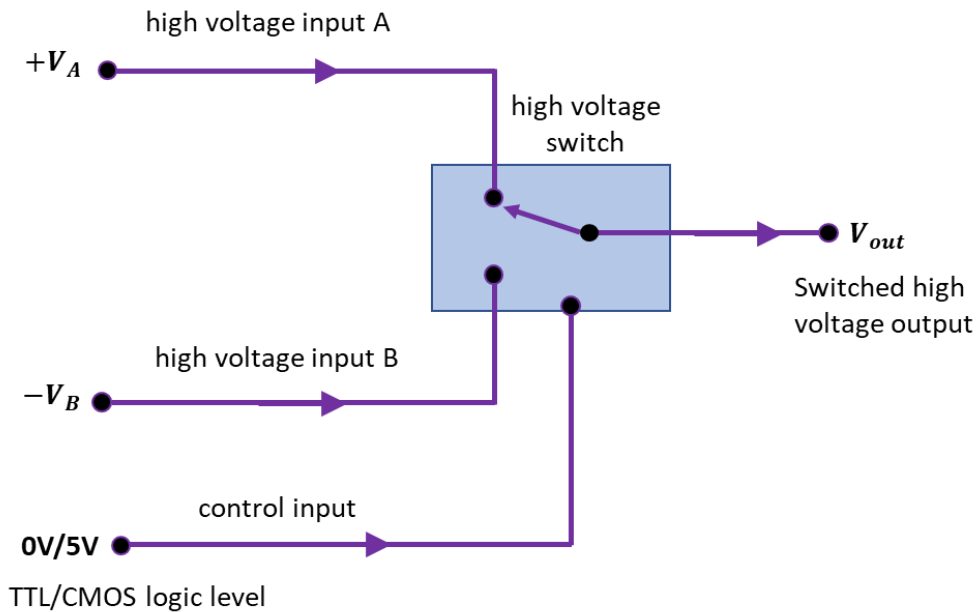
Figure 1: Schematic of the high voltage fast switch
